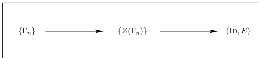
Figure 1: The construction of symbolic operators.
